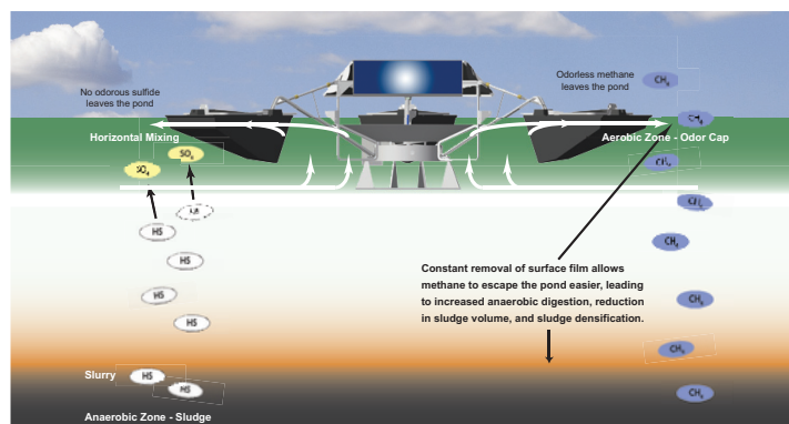
Figure 2. Odor-cap an anaerobic pond. Only the top two or three feet of the pond is mixed, effectively "capping" the anaerobic waters below.
