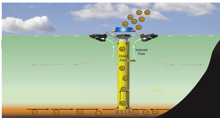
Figure 3: De-gassing a deep-water industrial pond. Deep dense water, along with hydrogen sulfide, is continuously drawn up to the surface of the pond and de-pressurized. Sulfides vent into the atmosphere at the distribution dish.
