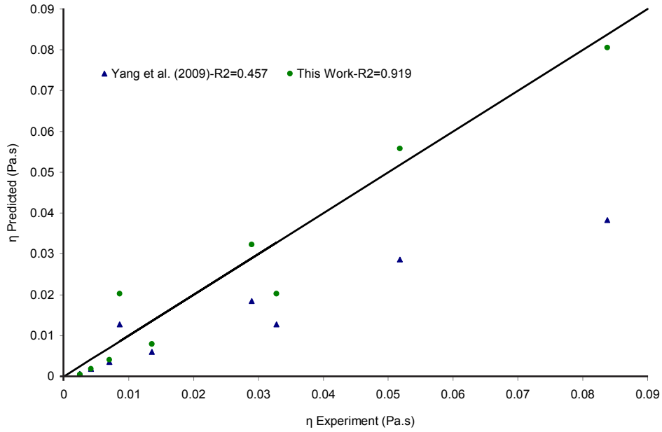
Fig. 3: Comparison of predicted data by Eq. (12) and Yang et al. (2009) with the experimental data
