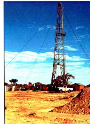
Drilling rig.
