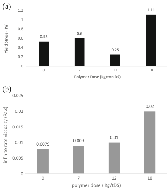
Fig. 17 Rheological model based parameters for different polymer dosage of digested sludge: a yield stress and viscosity (Herschel–Bulkley) and b infinite-rate viscosity (Sisko)
