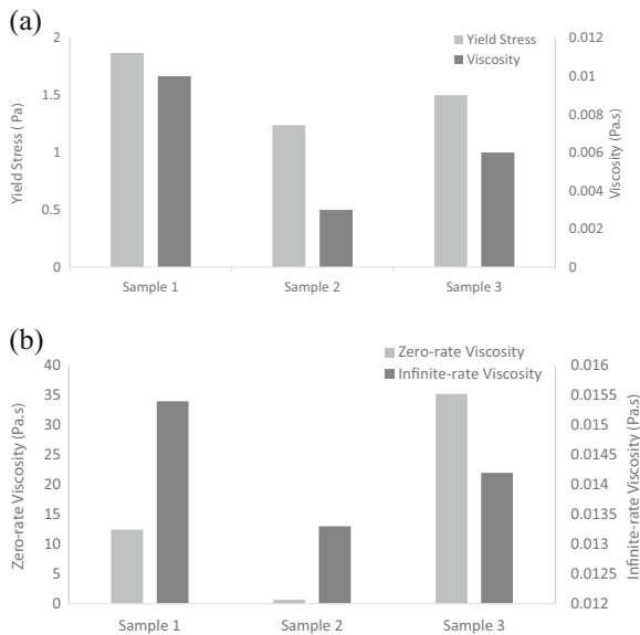
Fig. 19 Rheological model-based parameters for different digested sludge at different storage times: a yield stress and viscosity (Herschel–Bulkley) and b zero-rate viscosity and infinite-rate viscosity (Cross)
