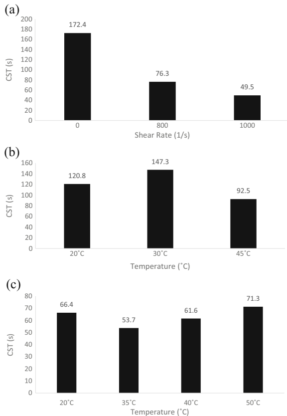
Fig. 10 Dewaterability of digested sludge due to the effects of a preshearing, b preshearing and temperature, and c preshearing and polymer conditioning at different temperatures
