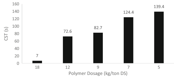
Fig. 14 Effect of polymer dose on digested sludge dewaterability
