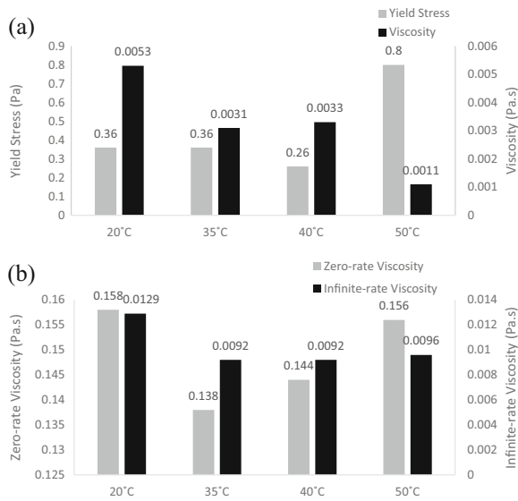
Fig. 7 Rheological model-based parameters for varying temperature of polymer conditioned digested sludge: a yield stress and viscosity (Herschel–Bulkley) and b zero-rate viscosity and infinite-rate viscosity (Cross)
