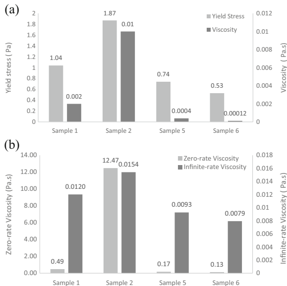
Fig. 4 Rheological model-based parameters for digested sludge from different collection days: a yield stress and viscosity (Herschel–Bulkley) and b zero-rate viscosity and infinite-rate viscosity (Cross)
