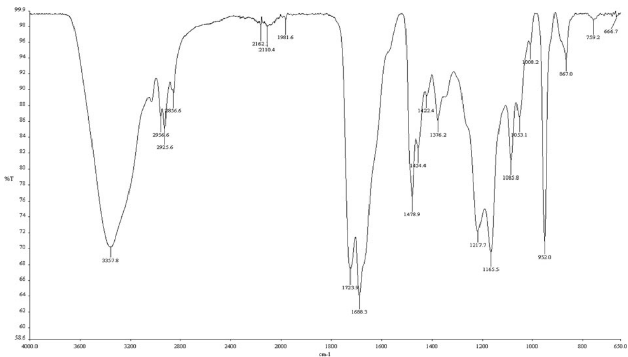
Fig. 2 FTIR spectra of the conditioning polymer
