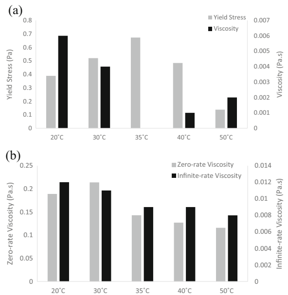
Fig. 9 Rheological model-based parameters for varying temperature of unconditioned digested sludge: a yield stress and viscosity (Herschel–Bulkley) and b zero-rate viscosity and infinite-rate viscosity (Cross)
