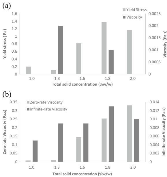
Fig. 12 Rheological model-based parameters for different total solid concentration of unconditioned digested sludge: a yield stress and viscosity (Herschel–Bulkley) and b zero-rate viscosity and infinite-rate viscosity (Cross)
